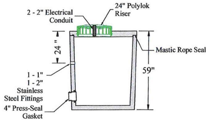
SECTION VIEW
