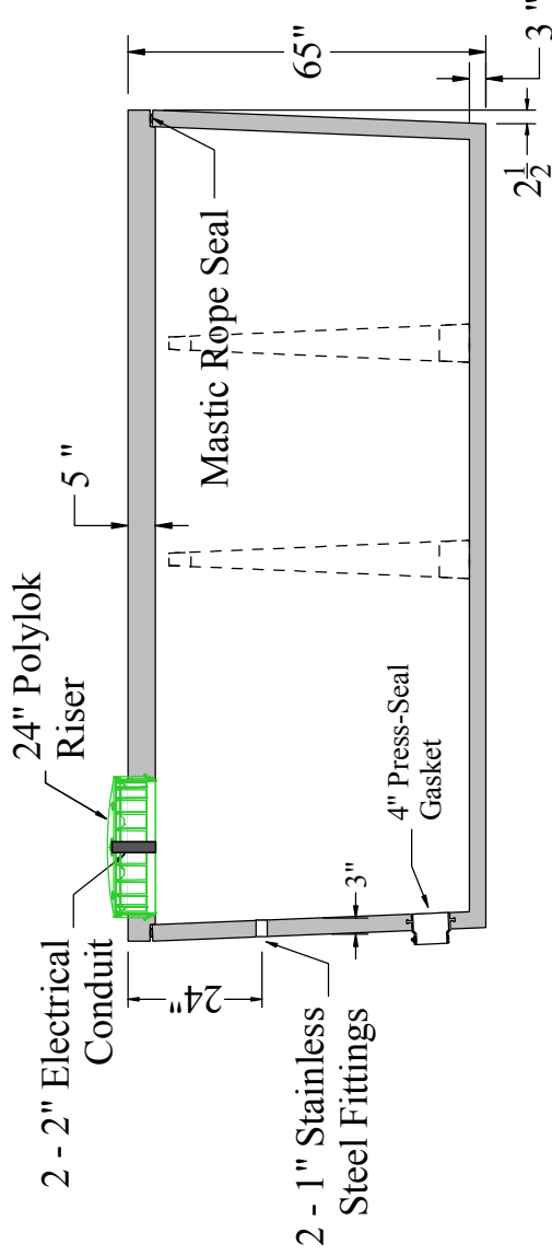
SECTION VIEW
