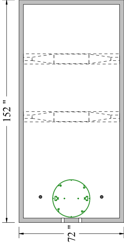
PLAN VIEW
