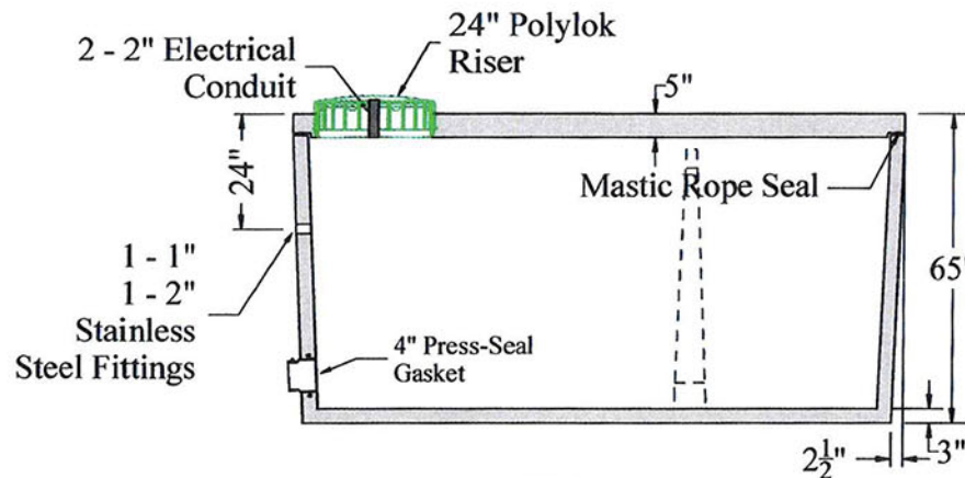
SECTION VIEW
