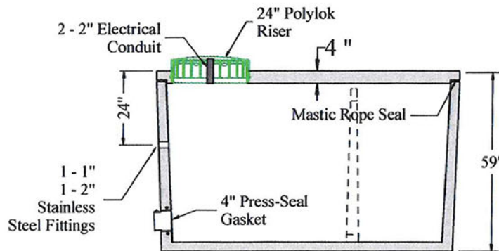
SECTION VIEW
